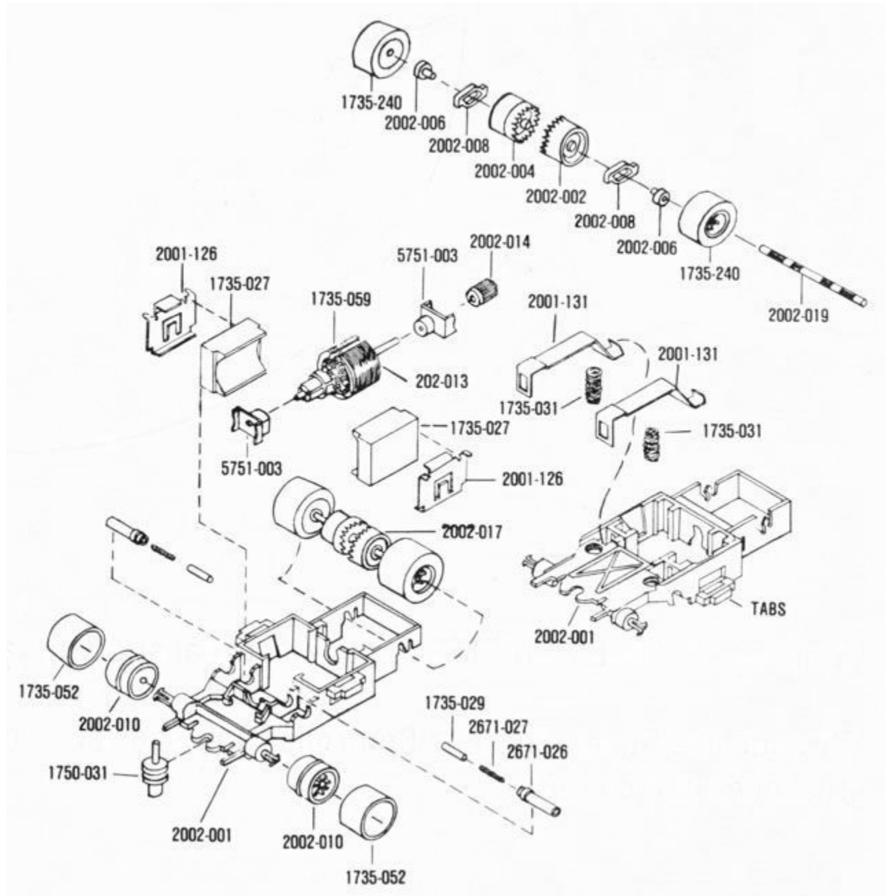
AFX Speed Shifter Schematic
